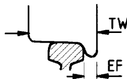
Tyre and railhead contours as per figure 1
